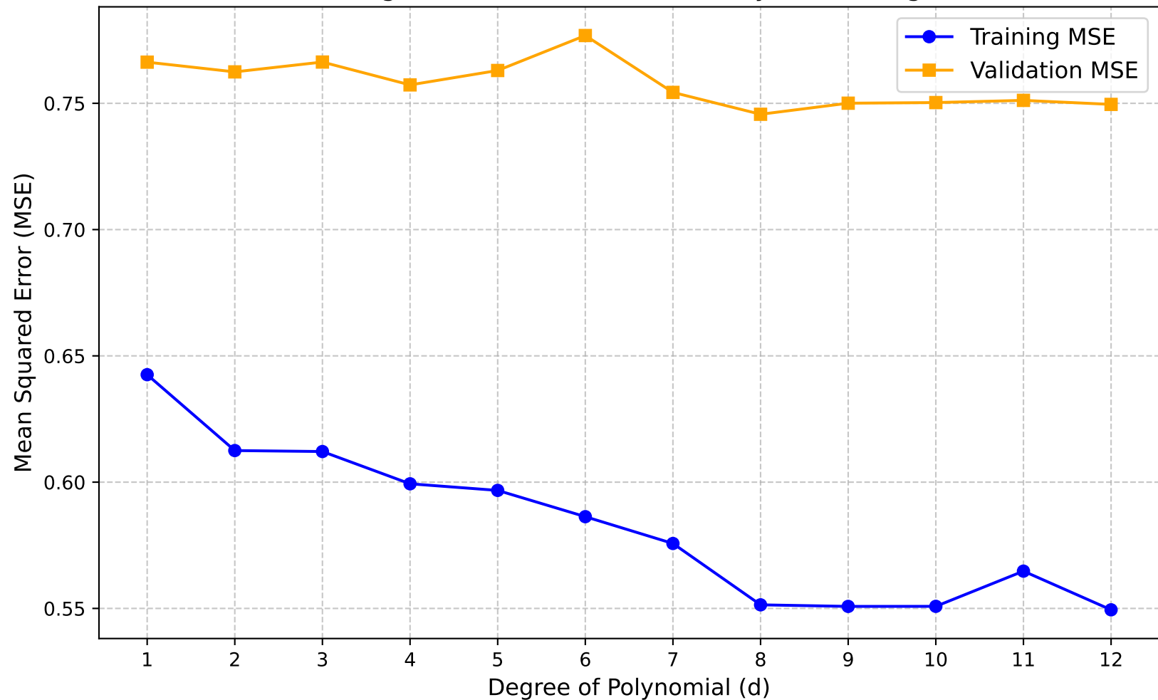
Training and Validation MSE vs. Polynomial Degree
